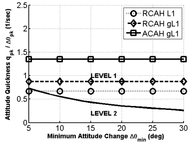
Figure 6. Vehicle dynamics model predicted pitch quickness
