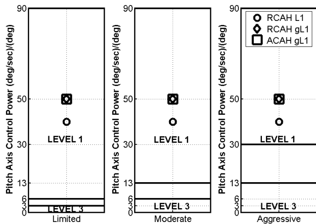
Figure 5. Large amplitude pitch response HQ characteristics
