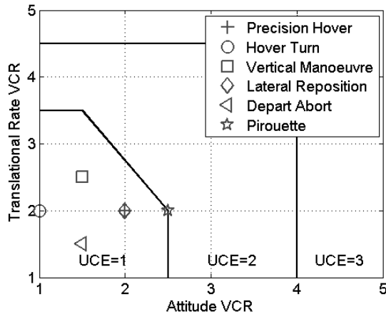
Figure 8. Useable cue environment for the tested MTEs
